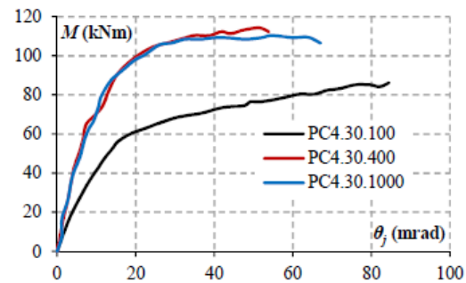
Figure 2.8: Moment-rotation curves for PC4.30 tests (Seco, 2019)
