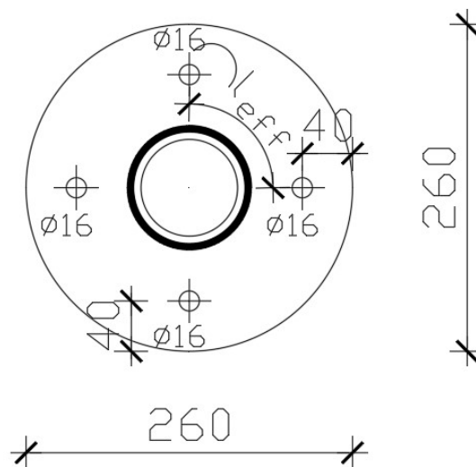
Figure 6.5. representation of plate with bolts
