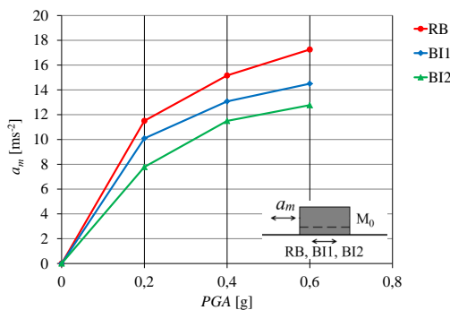
Figure 2.16 The peak acceleration a_m envelope of all excitation applied on the M_0 based on RB , BI1 , and BI2
