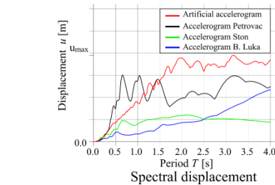
(b) Spectral values of adopted accelerograms
