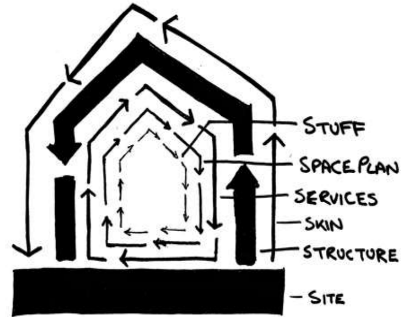
Izvor: https://en.wikipedia.org/wiki/Shearing_layers
