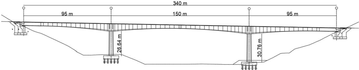
Figure 38. Vranduk 2 left bridge longitudinal section
