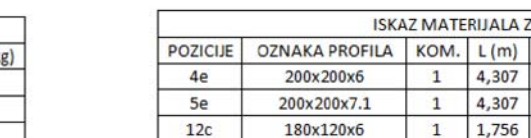
POZ 12c 180x120x6, L= 1756 mm, kom 1
