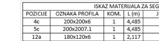
POZ 12a 180x120x6, L= 2117 mm, kom 1
