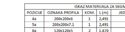
POZ 8a 120x120x5, L= 1470 mm, kom 2
