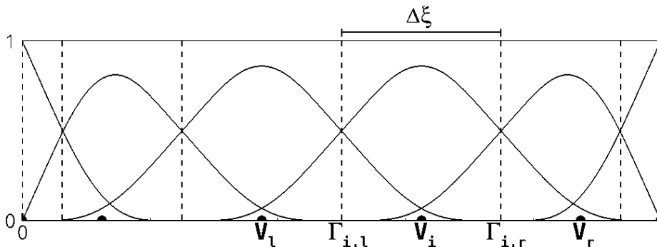
FIGURE 6.4: Nonoverlapping control volume scheme for one-dimensional case.
