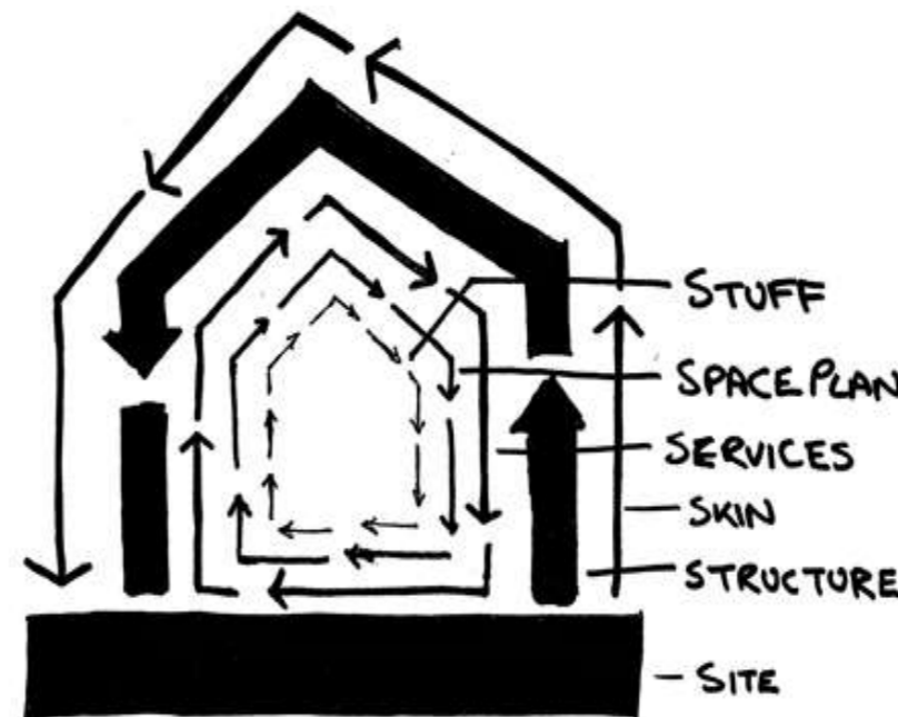
Izvor: https://en.wikipedia.org/wiki/Shearing_layers
