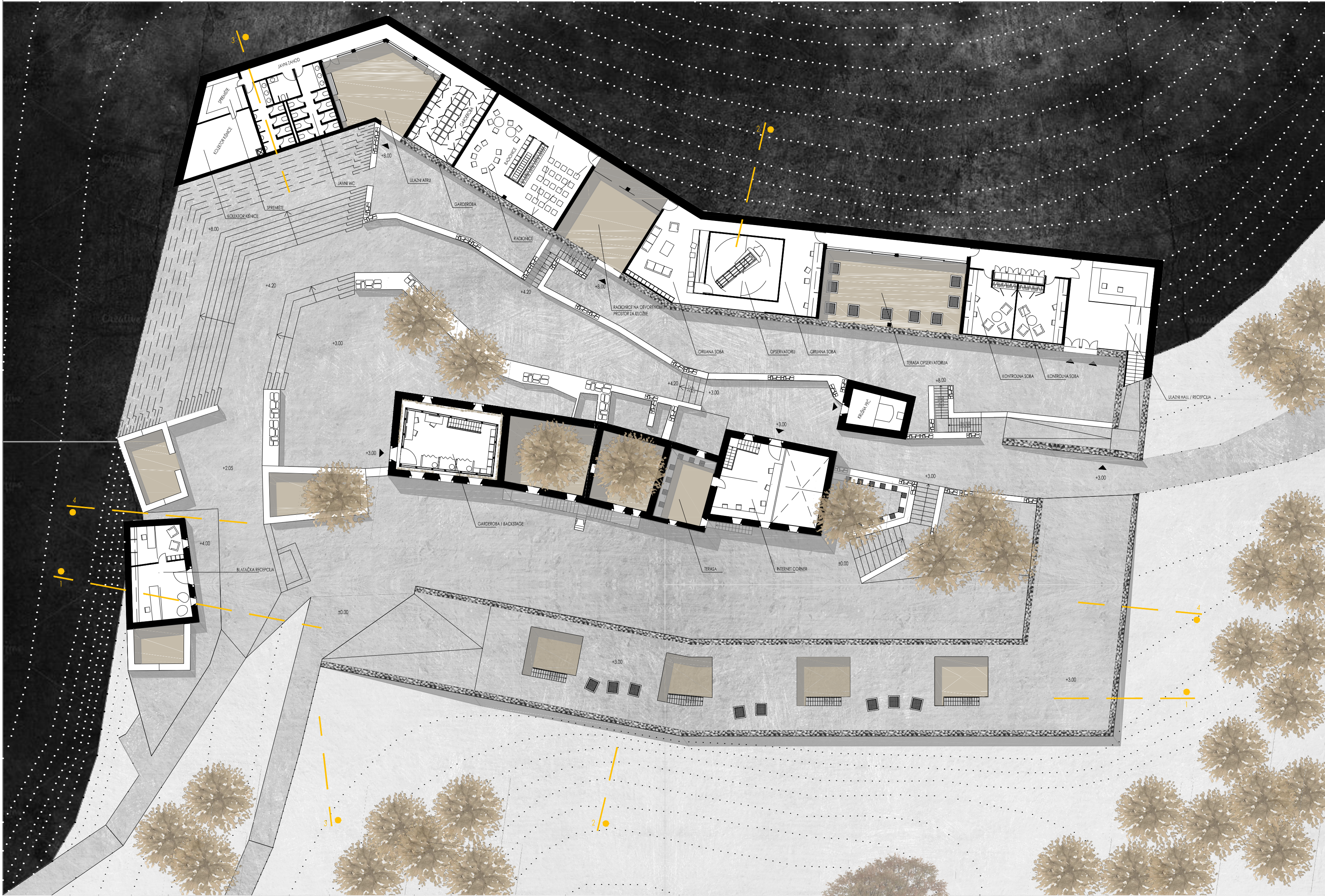
TLOCRT ±8.00
