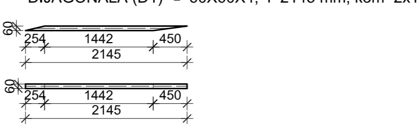
DIJAGONALA (D1) 60X60X4, l=2145 mm, kom=2x11
