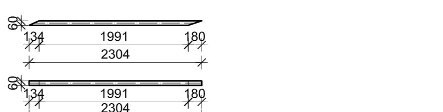
DIJAGONALA (D3) 60X60X4, l=2304 mm, kom=2x11
