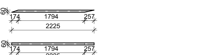
DIJAGONALA (D2) 60X60X4, l=2225 mm, kom=2x11
