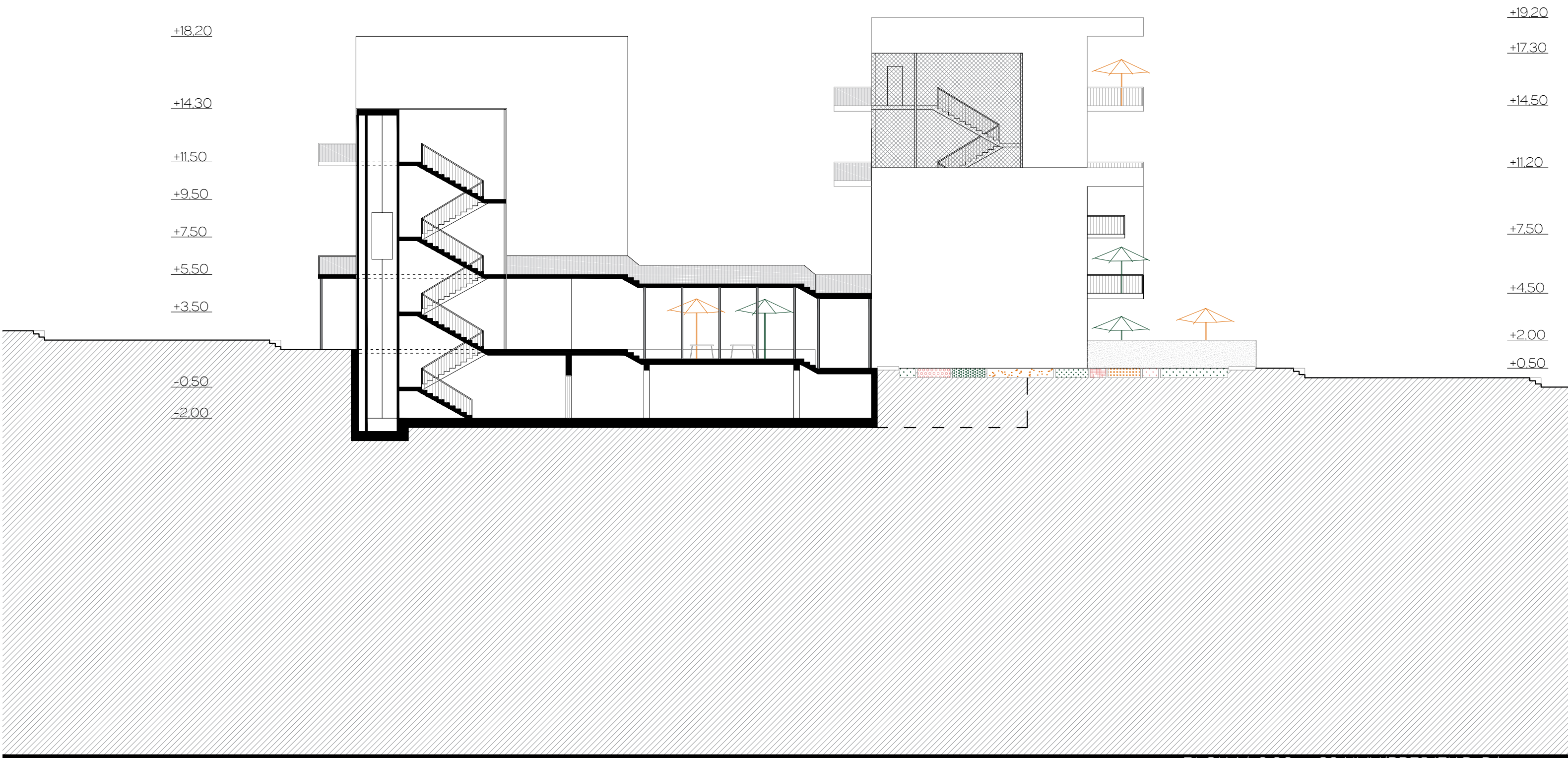
BLOK A/±0.00 = +20 NMV/PRESJEK D-D/
