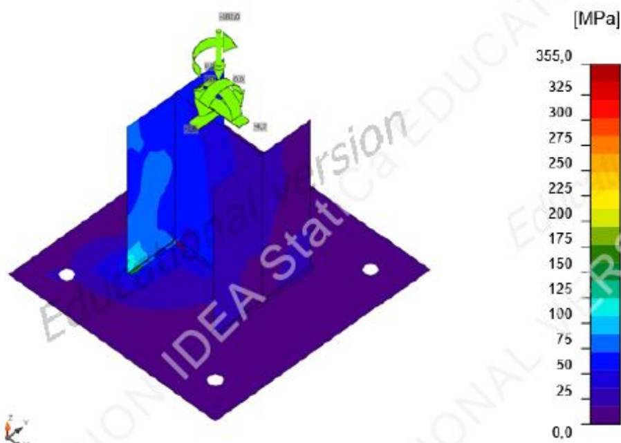
Equivalent stress, GSN16(9)
