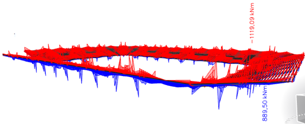
My (kNm)
