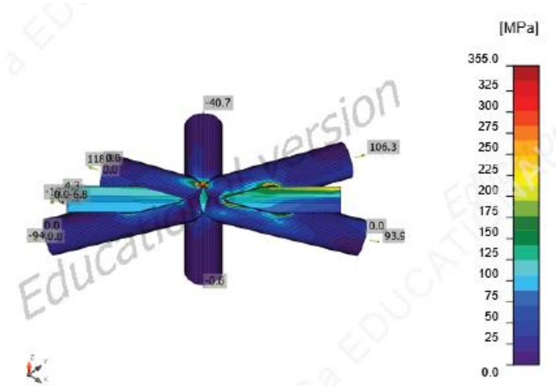
Equivalent stress, GSN2(2)
