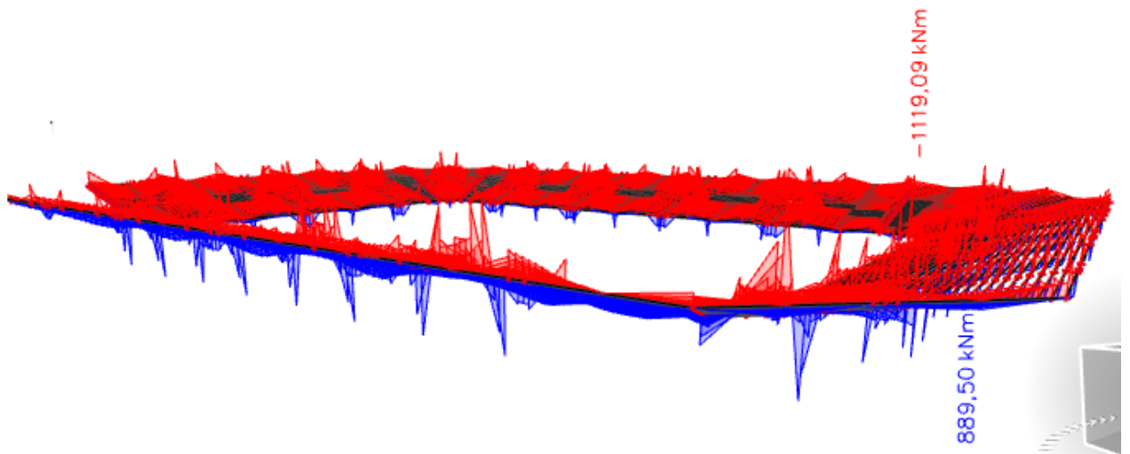
My (kNm)
