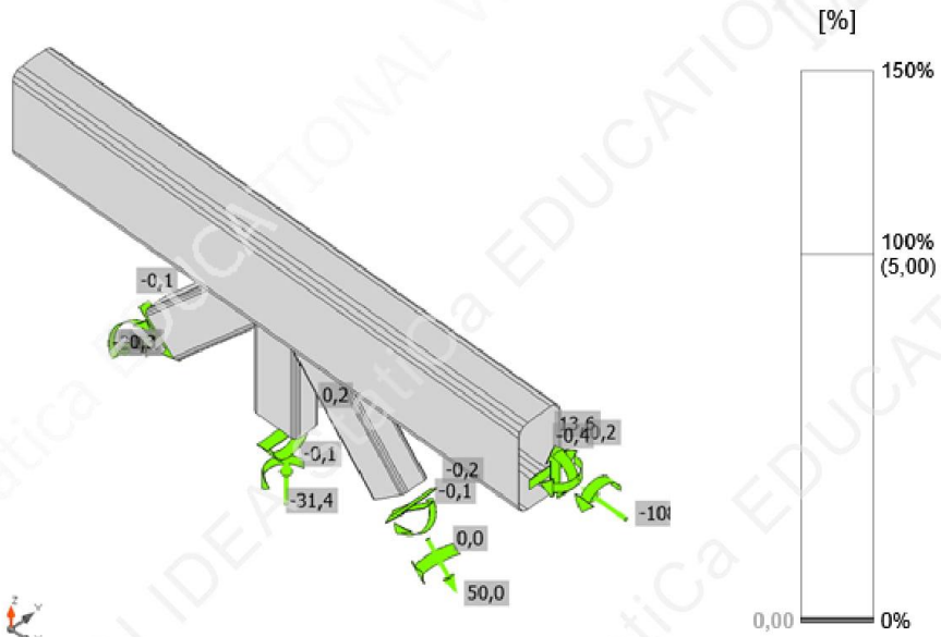
Strain check, ULS-Set(7)
