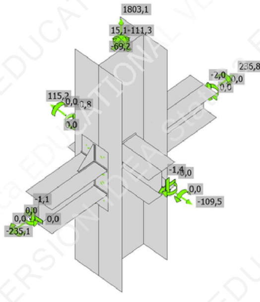
Overall check, ULS-Set(6)
