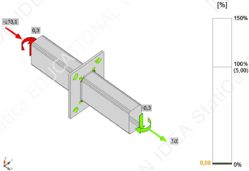
Strain check, LE1
