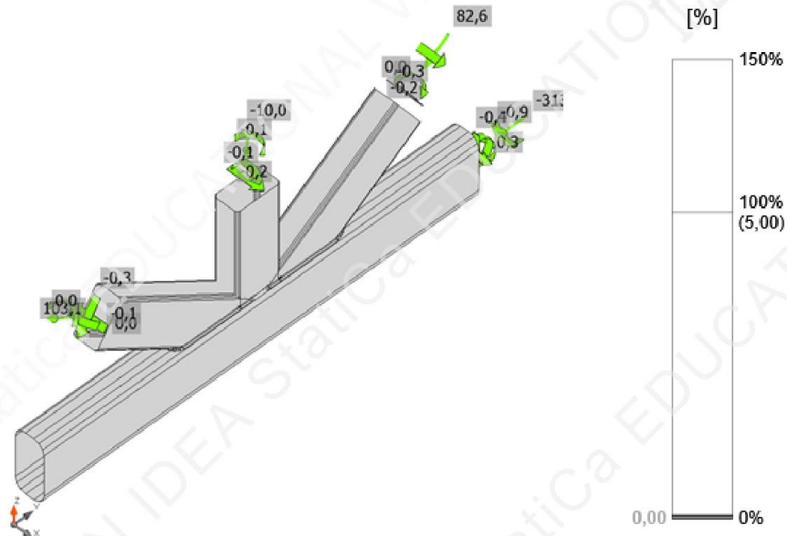
Strain check, ULS-Set(10)
