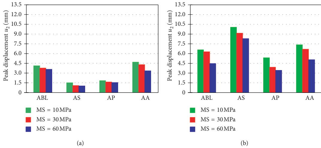
FIGURE 19: The effect of pebble layer compaction on peak horizontal displacement u_2 . (a) PGA = 0.2\text{ g} . (b) PGA = 0.6\text{ g} .
