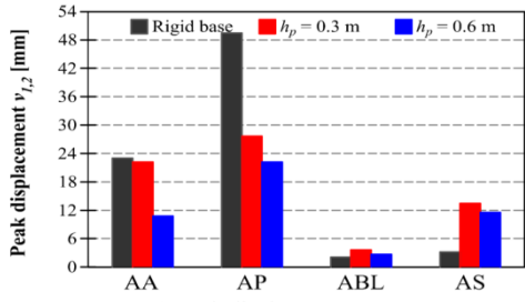
e) Peak displacement v_{I,2} [mm]
