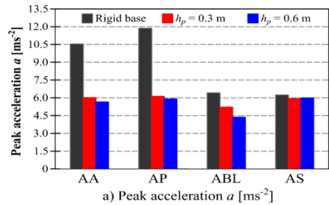
a) Peak acceleration a [ms -2 ]
