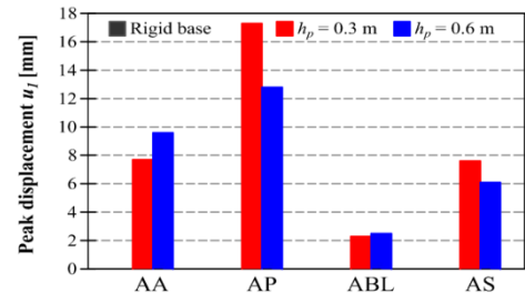
c) Peak displacement u_I [mm]
