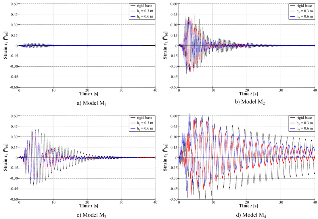
Figure 13 - Vertical strain on the right bottom side of the steel column \varepsilon_1 for accelerogram AS
