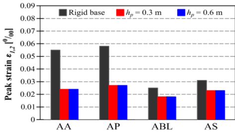
b) Peak strain \epsilon_{I,2} [‰]
