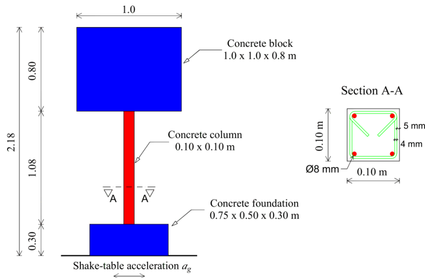
Figure 2.4 Model of cantilever concrete column tested on aseismic layer ASL-1
