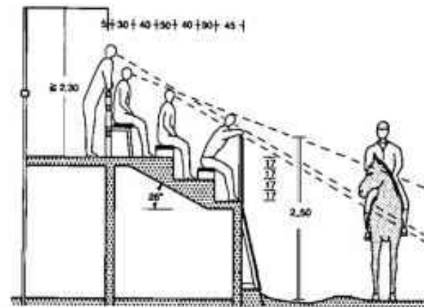
11 Tribina s ophodom
