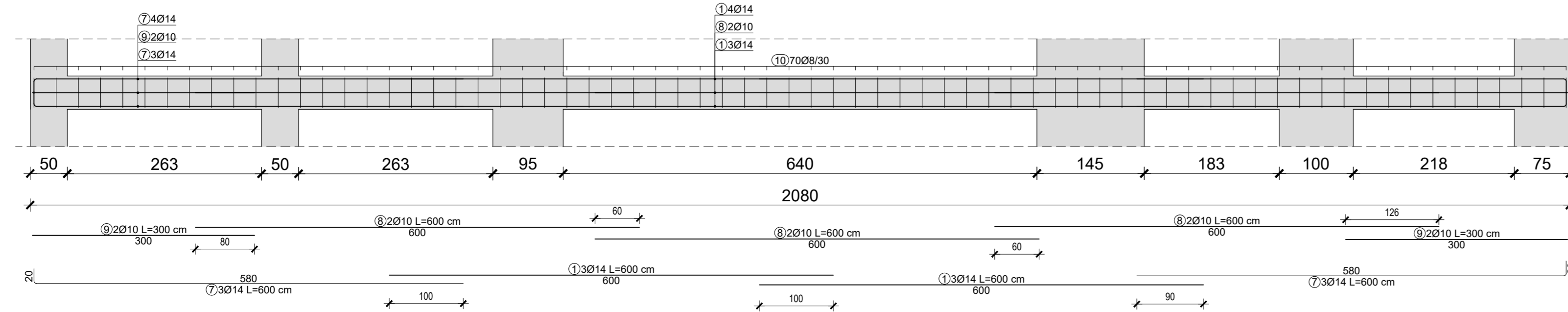
greda u osi C b/h=25/45 cm
