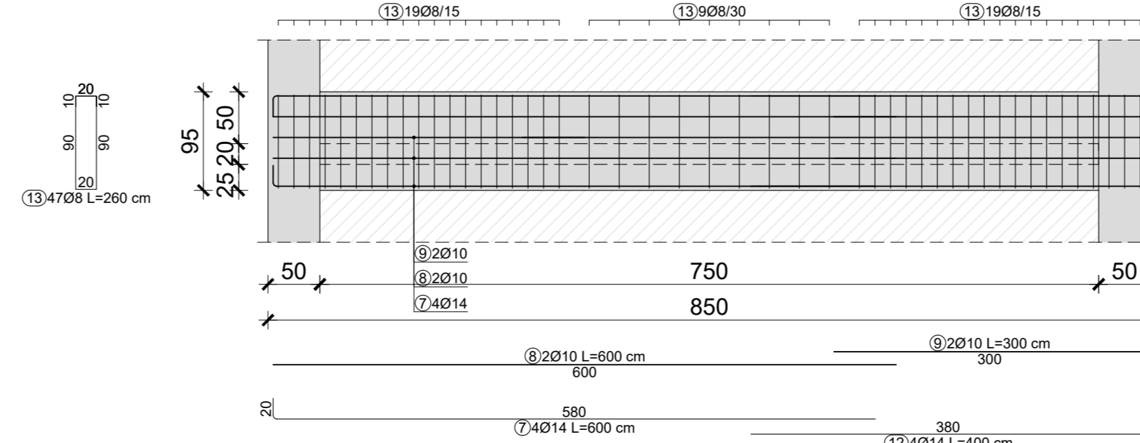
parapetna greda u osi 6/A-C, b/h=25/95 cm
