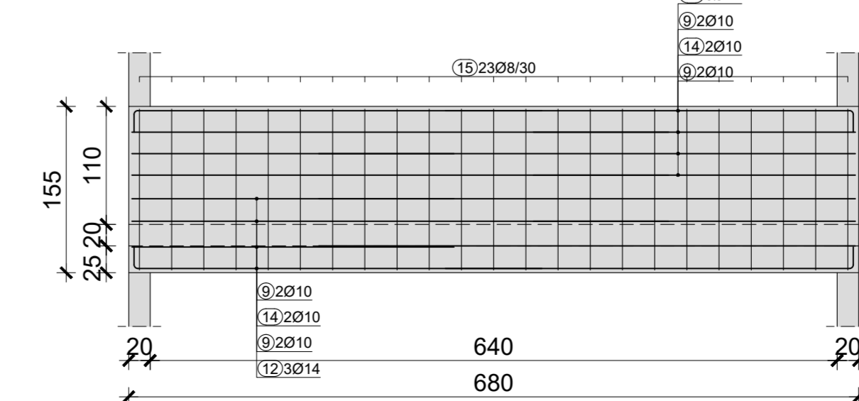
parapetna greda u osi D/3-4, b/h=25/155 cm
