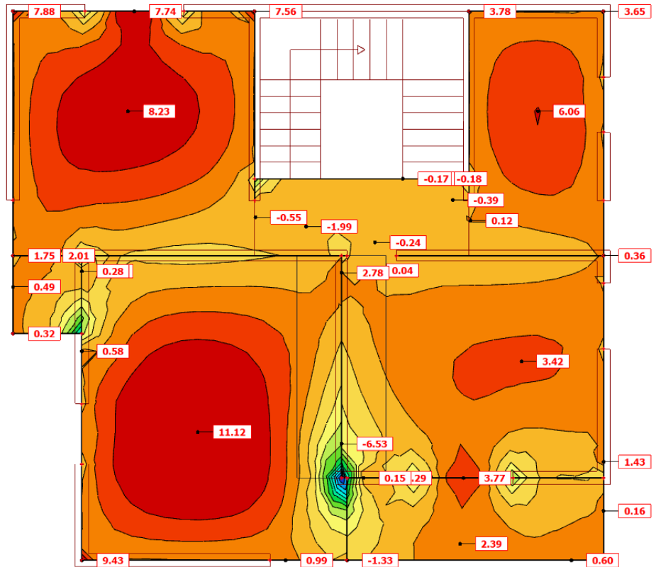
Moment m_x
