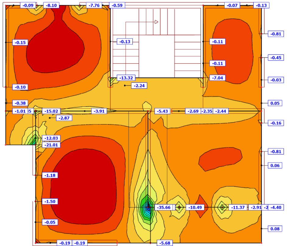
Moment m_x
