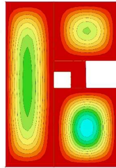
Progibi ploča. U_z (mm) – GSU – 2 ( \delta_{\max,d} \leq L/1250 )
