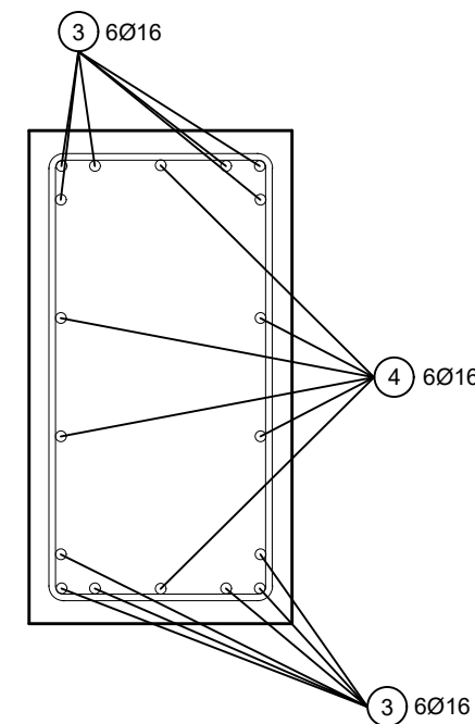
Presjek 1-1 MJ 1:12.5
