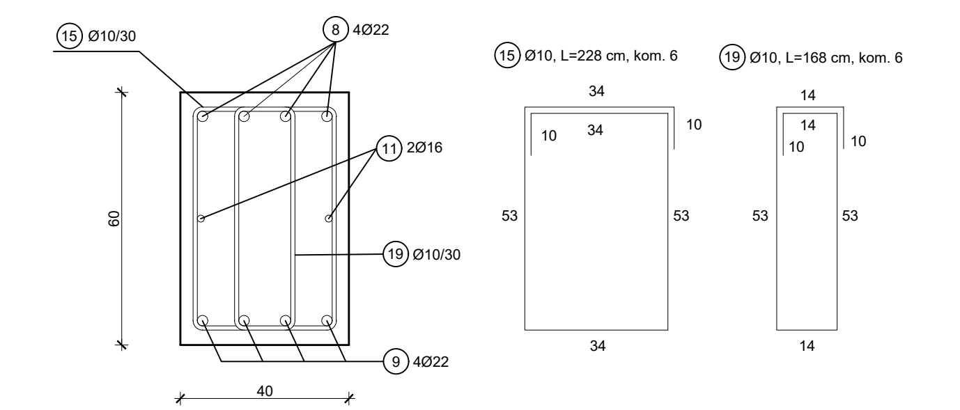
PRESJEK 5-5 MJ 1:12.5
