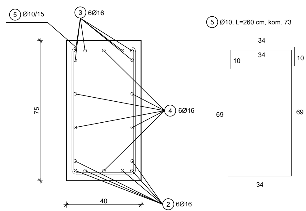
PRESJEK 4-4 MJ 1:12.5
