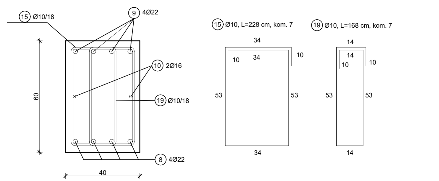
PRESJEK 6-6 MJ 1:12.5
