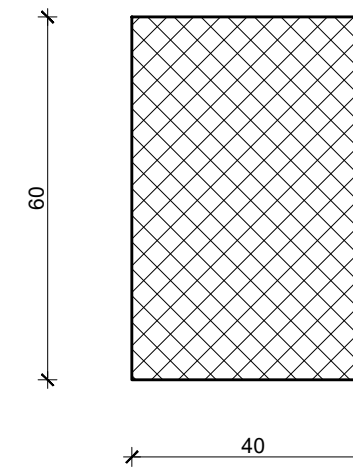
PRESJEK 4-4 MJ 1:12.5
