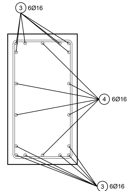
Presjek 1-1 MJ 1:12.5
