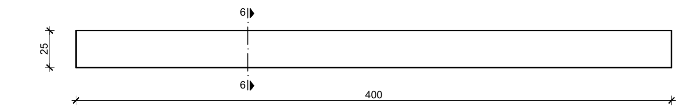
Presjek 6-6; MJ 1:12.5
