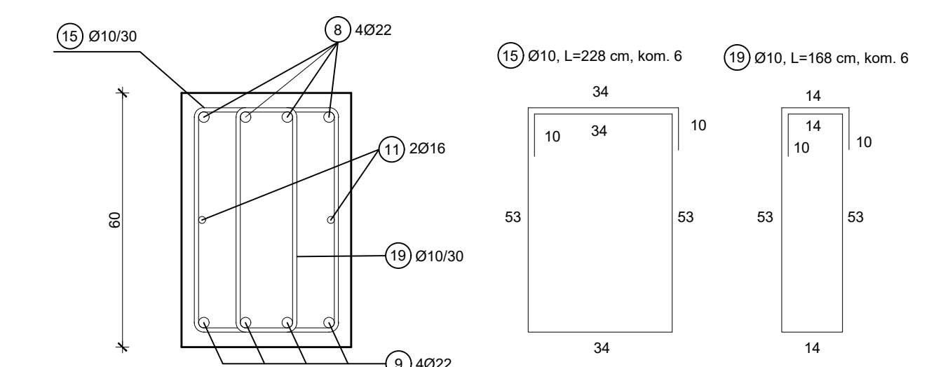
PRESJEK 5-5 MJ 1:12.5
