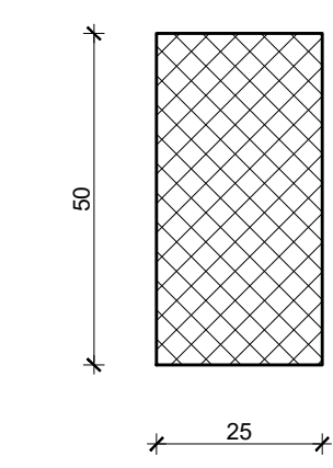
Presjek 6-6; MJ 1:12.5
