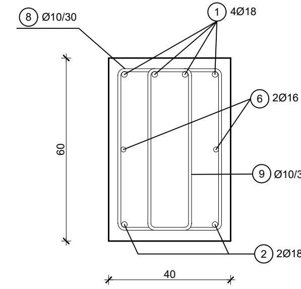
PRESJEK 2-2 MJ 1:12.5
