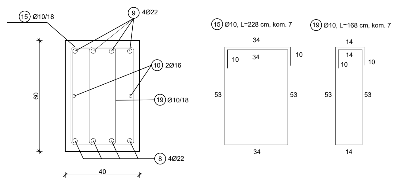
PRESJEK 6-6 MJ 1:12.5
