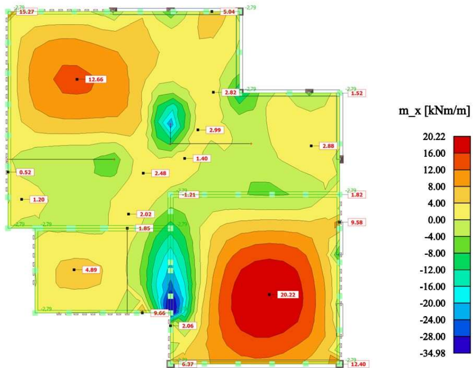
Moment m_x
