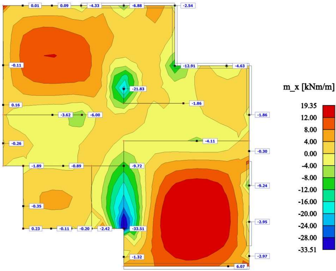
Moment m_x
