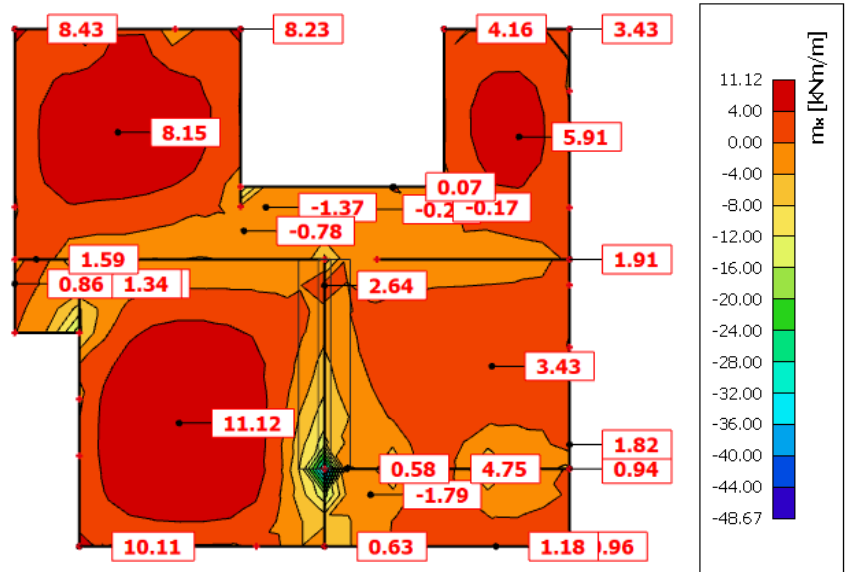
Moment m_x
