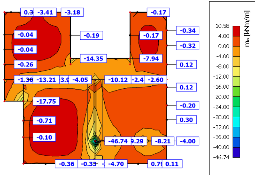
Moment m_x
