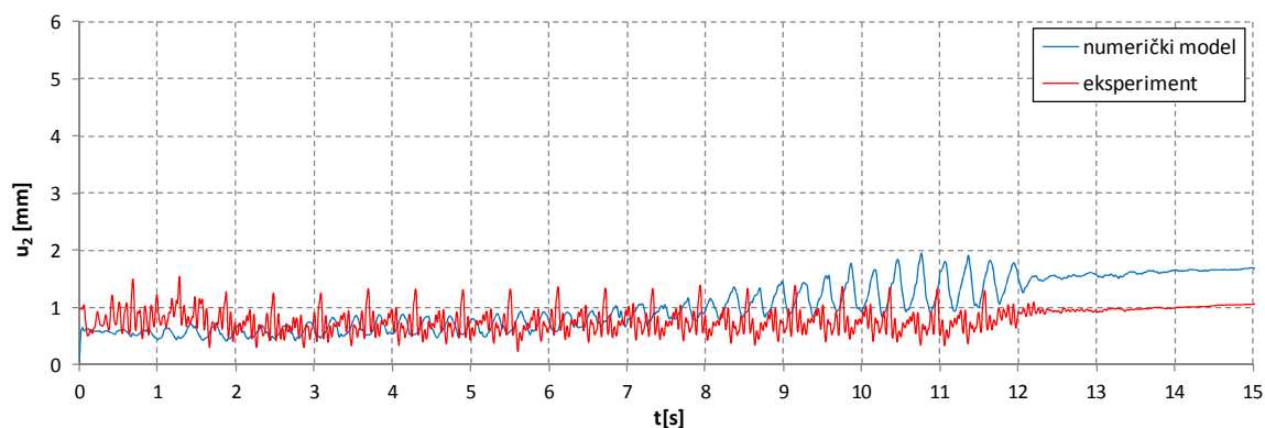
(a) a_0=0.1g
