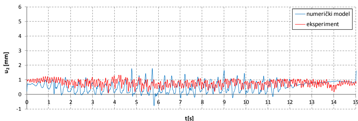
(c) a_0=0.5g
