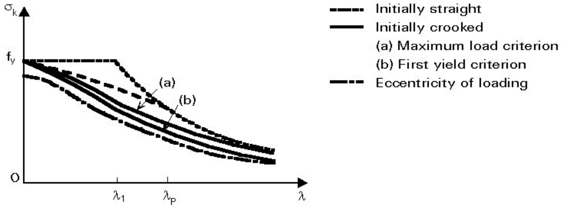
Figure 22: Strength curves
