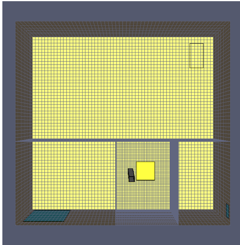
Figure 31: Computational domain
