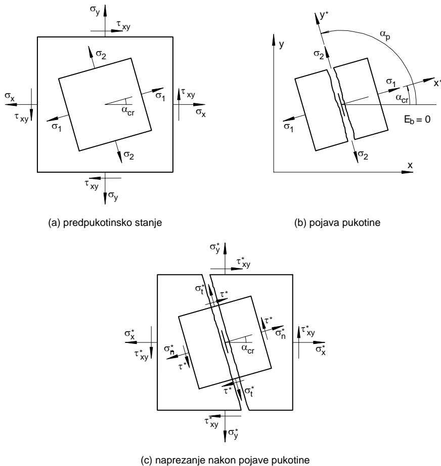
Crtež 2.19 - Model pukotina, lit. [D.1]
