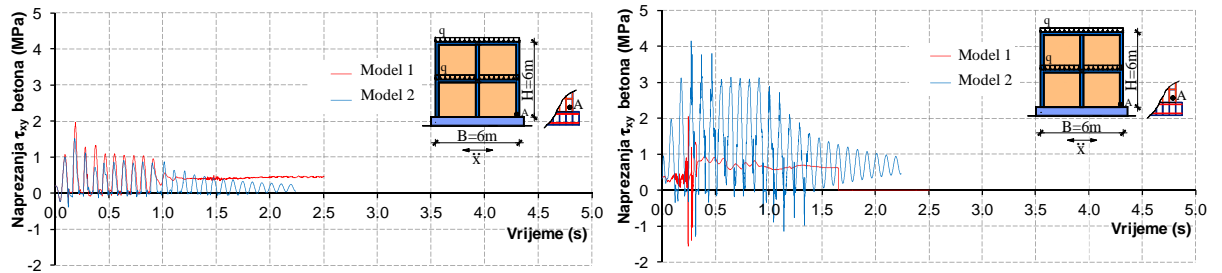
(ii) Zid CM_2
