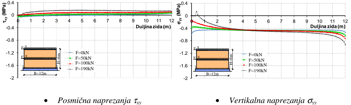
(iii) Zid URM 3
